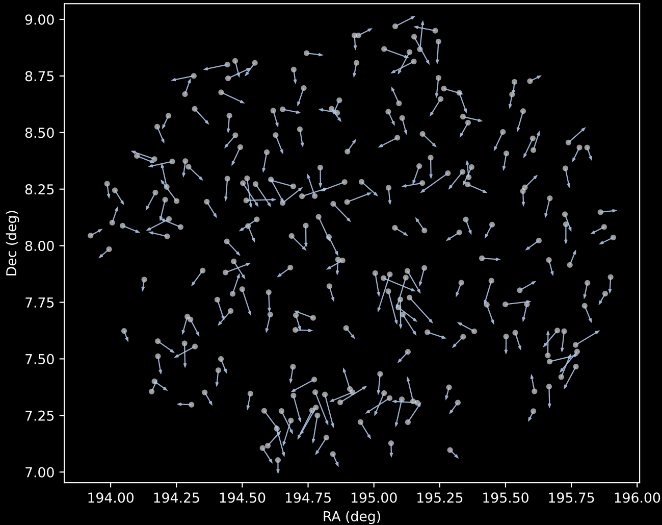
GALAH DR4 Cluster 1 Proper Motion Vectors (n=228)
