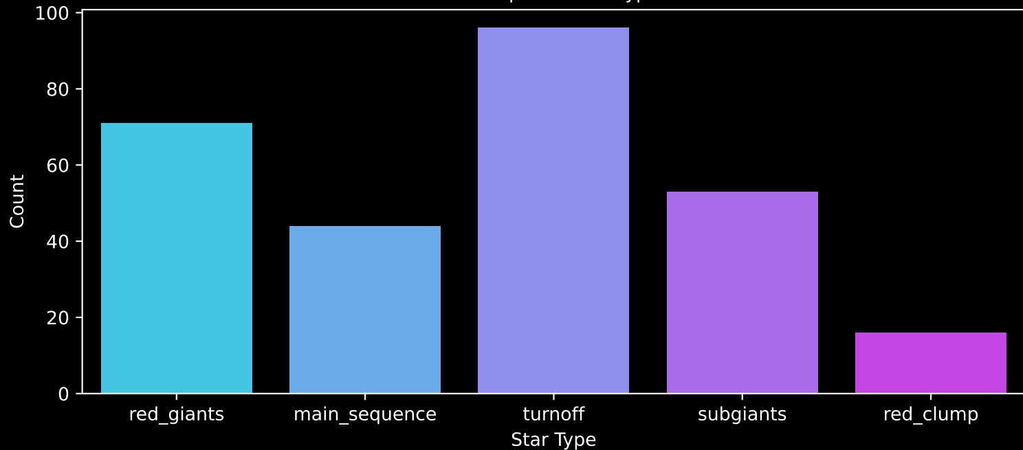
GALAH DR4 Field: [9470] Count plot of Star Type
