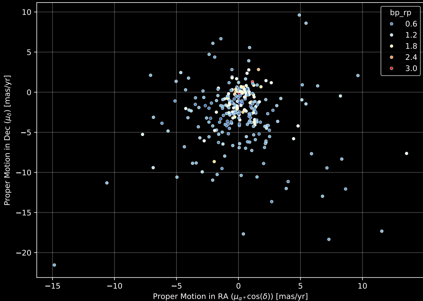
GALAH DR4 Field: [9470] Proper Motion Diagram (n= 280)
