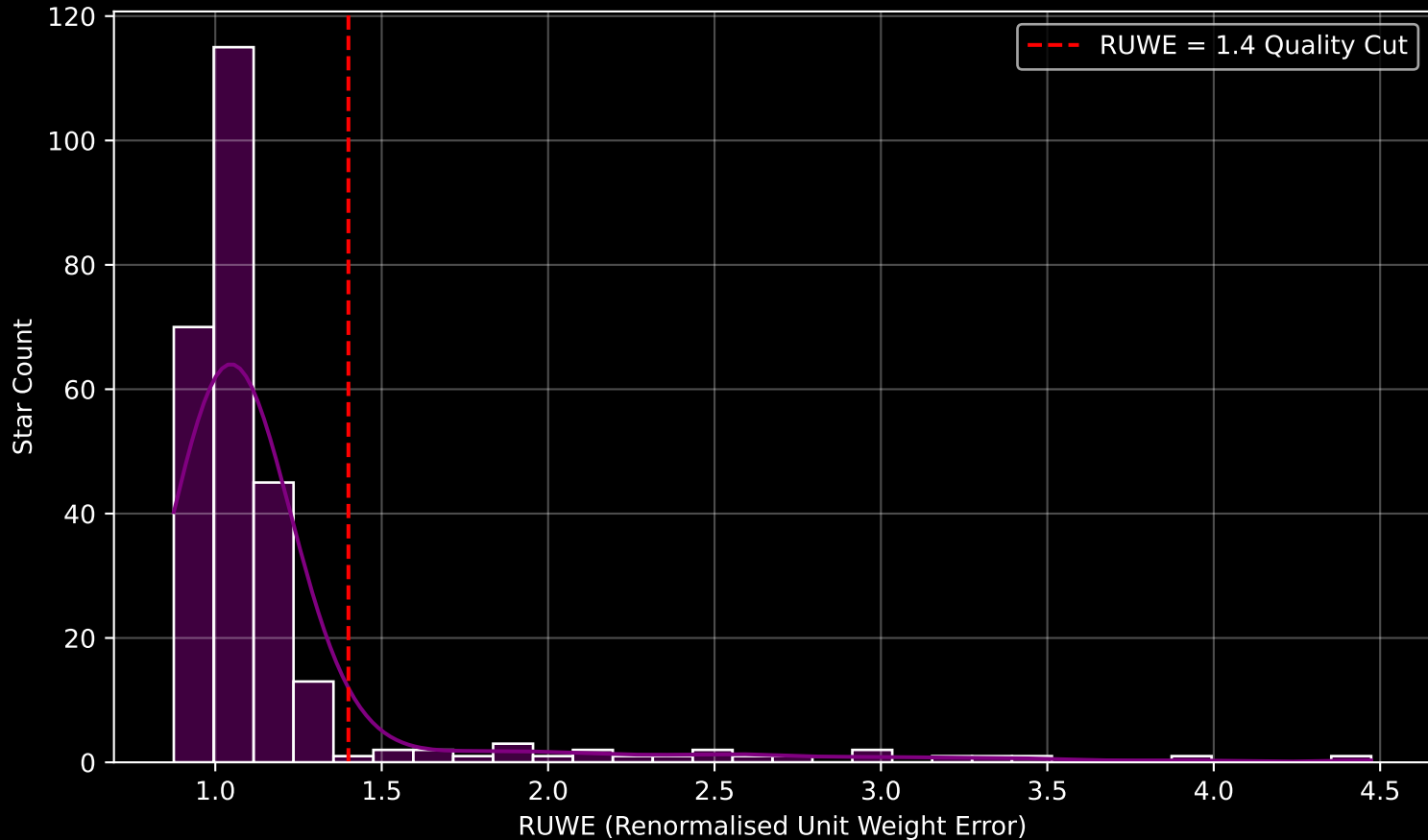
GALAH DR4 Field [9470] RUWE Distribution (n= 268)
