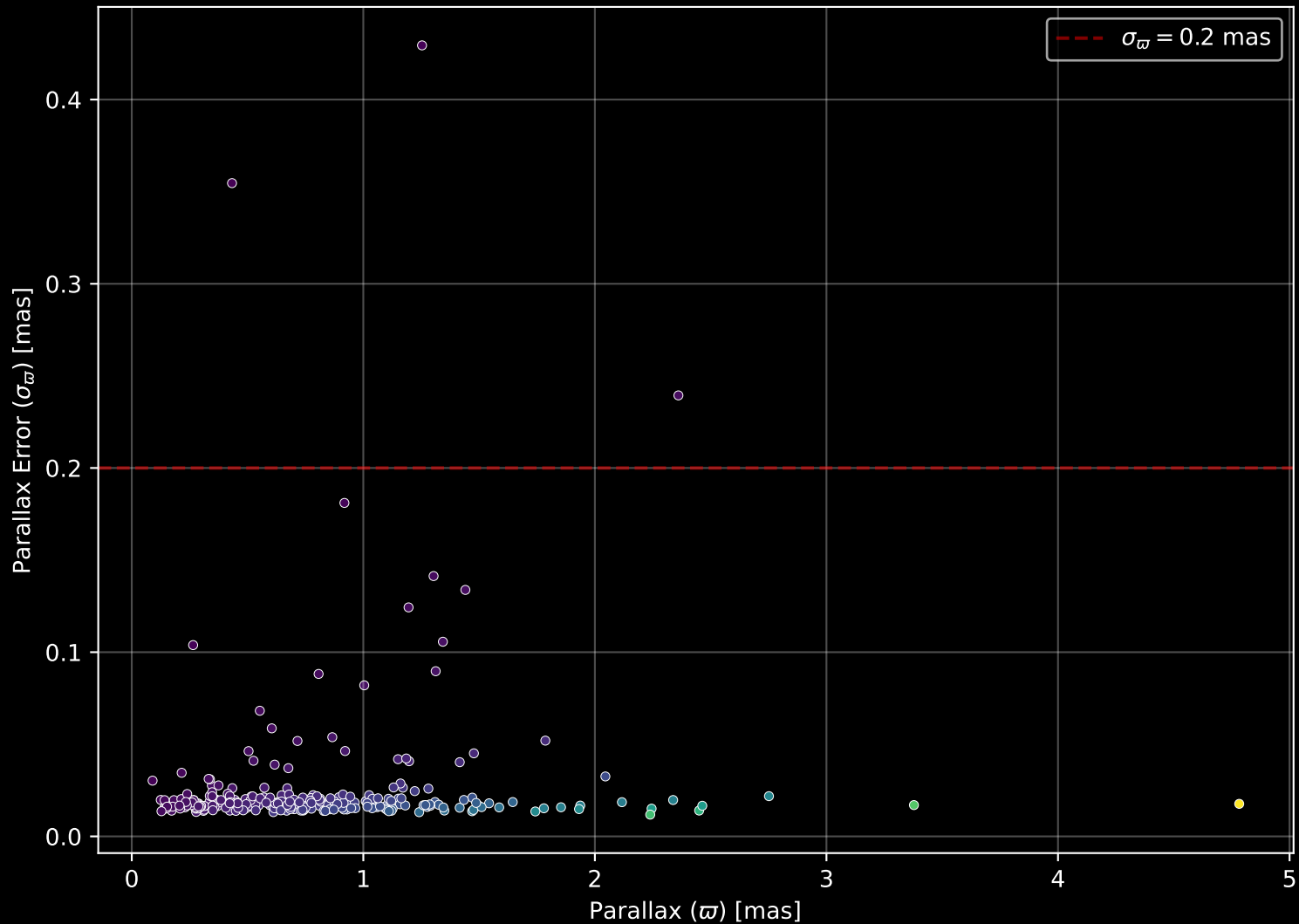
GALAH DR4 Field: [9470] Parallax Quality (n= 280)
