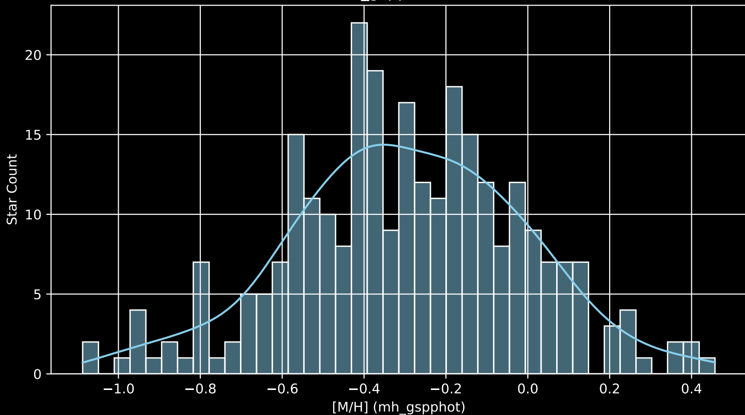
GALAH DR4 Field: [9470] [M/H] (mh_gspphot) (n= 280)
